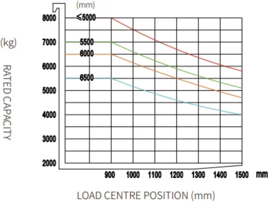
EFL803-HV-9 RATED CAPACITIES AND LOAD CENTERS GRAPH
