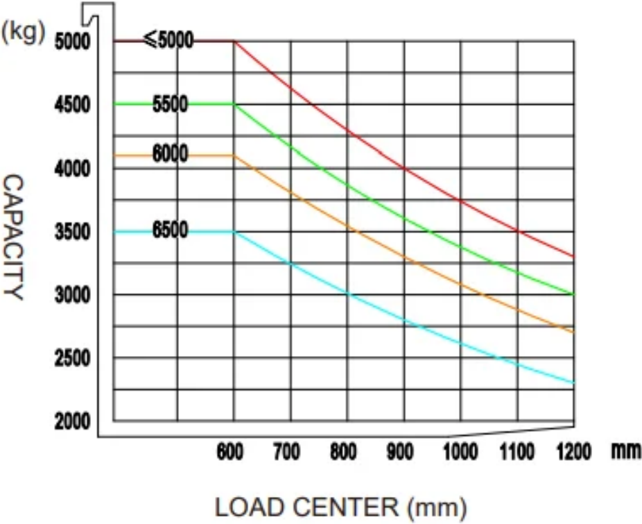
EFL503-HV-6 RATED CAPACITIES AND LOAD CENTERES GRAPH
