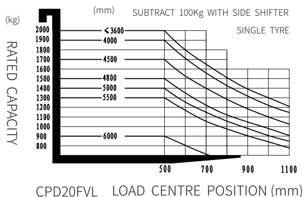
RATED CAPACITIES AND LOAD CENTERS GRAPH
