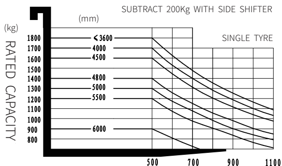
RATED CAPACITIES AND LOAD CENTERS GRAPH
